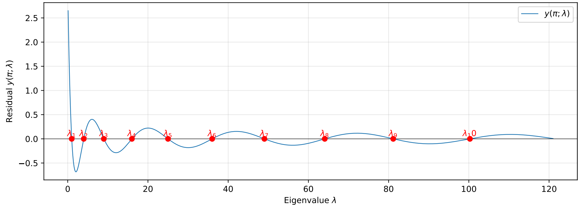
Residual sweep on clustered grid (n=100, 70%/30%) for 10 eigenvalues
